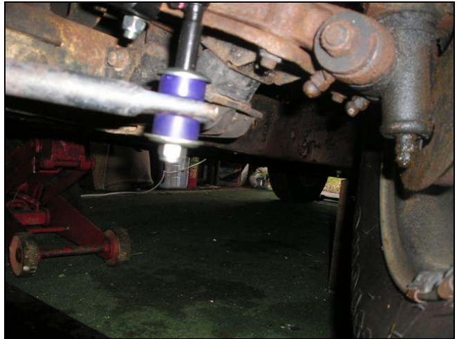
Fig 2: Assembly of drop link bushes & washers onto ARB.
