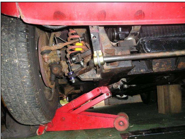
Fig 3: ARB centre mounts fitted to bumper irons
