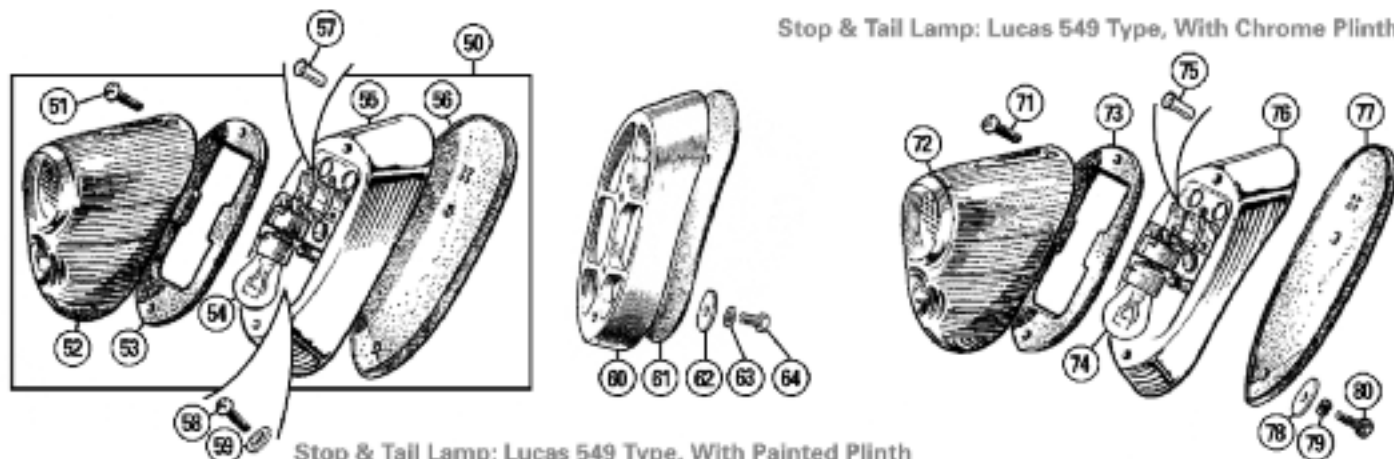
Stop &amp; Tail Lamp: Lucas 549 Type, With Painted Plinth
