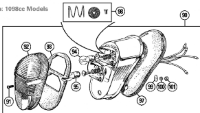
Stop &amp; Tail Lamp: Lucas 549 Type, With Painted Plinth
