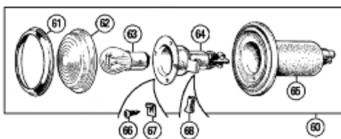
Side &amp; Indicator Lamp Assembly (from (c) 224166) - Lucas 488
