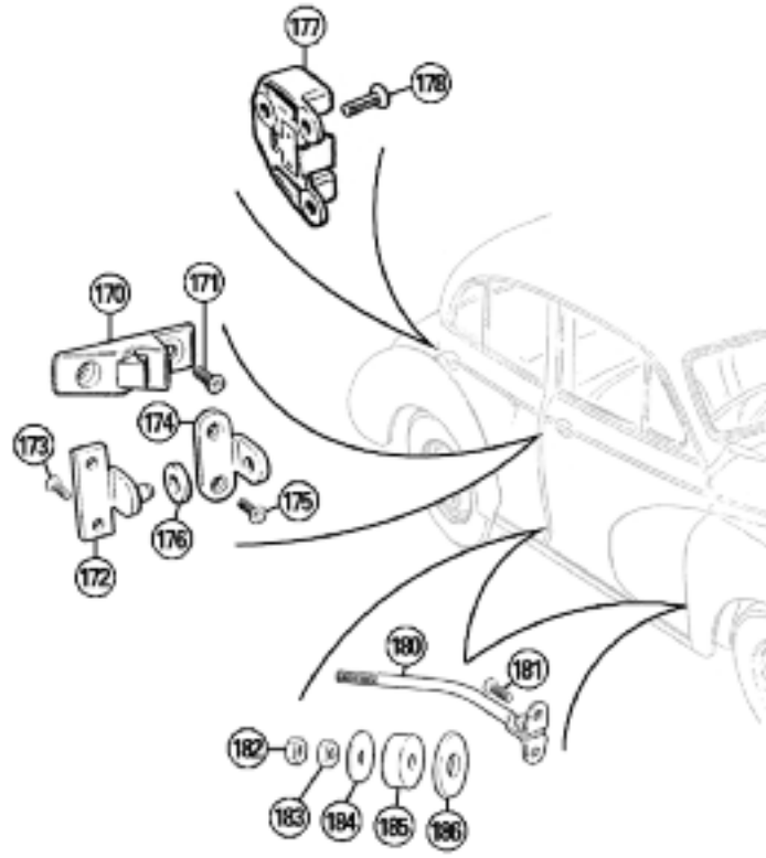
Catches &amp; Checkstraps
