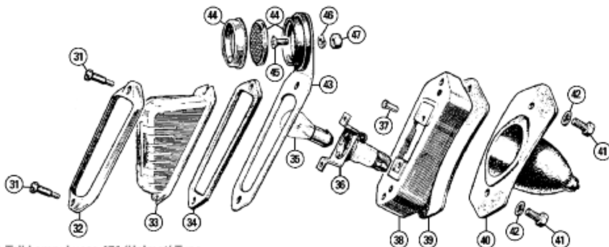
Stop &amp; Tail Lamp: Lucas 471 'Helmet' Type
