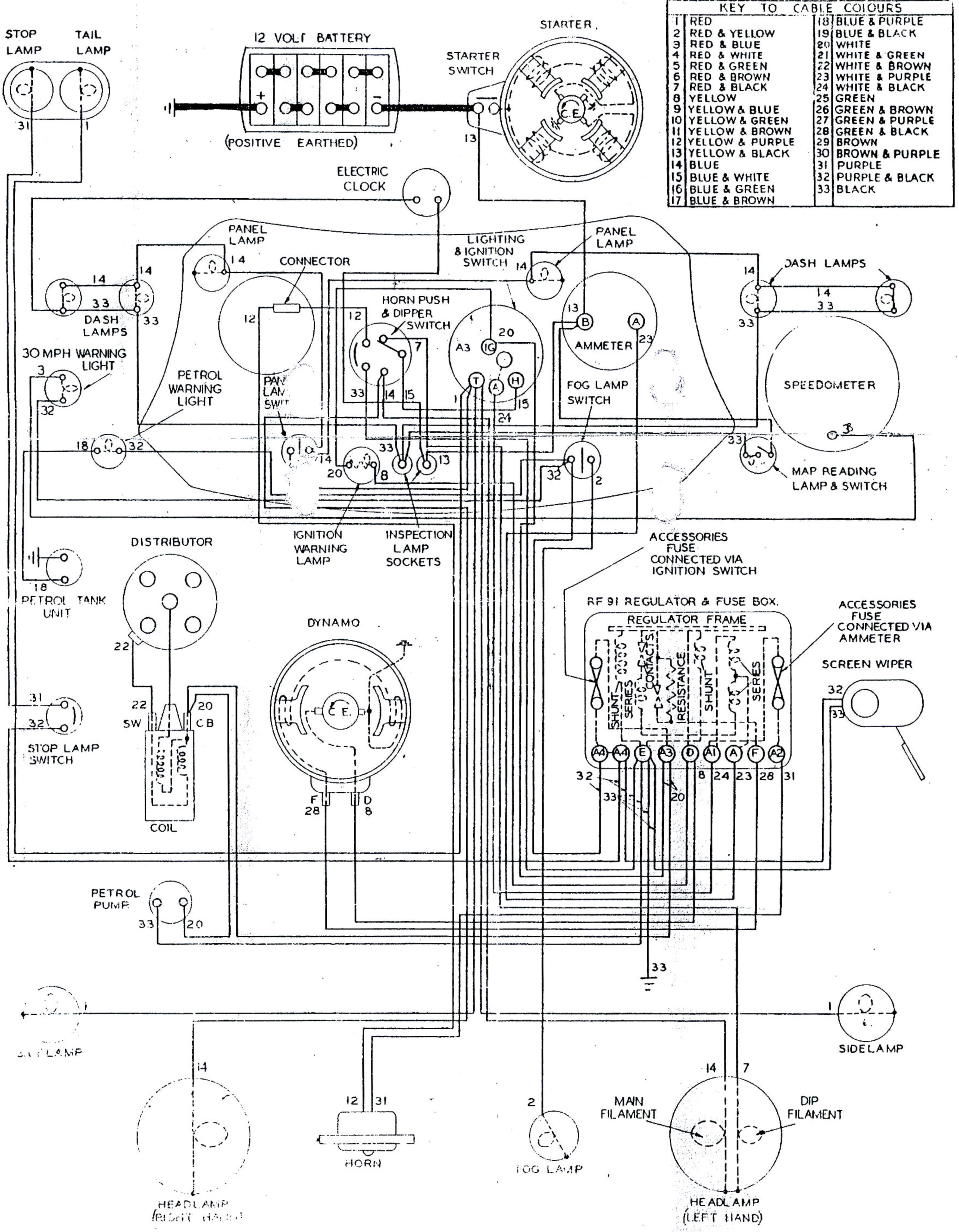
Illustration No. 50.—Diagram of electrical wiring system.
