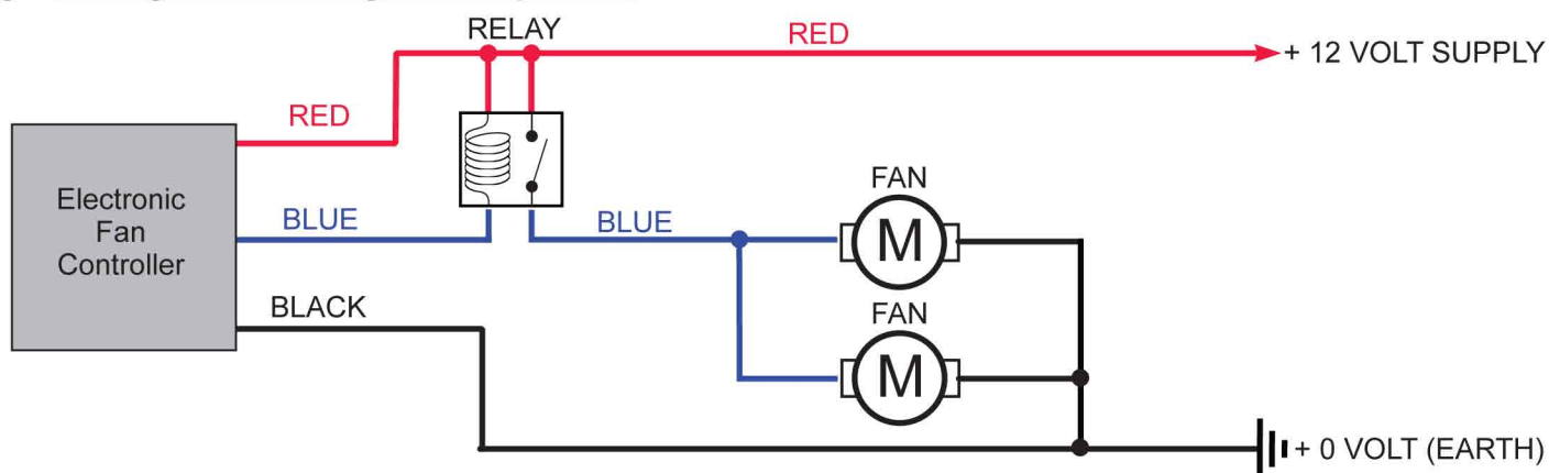
Fig.6 Wiring twin cooling fans in parallel
